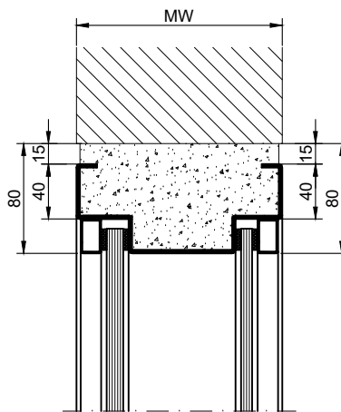
Blockzarge
