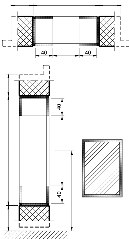
flush glazing
