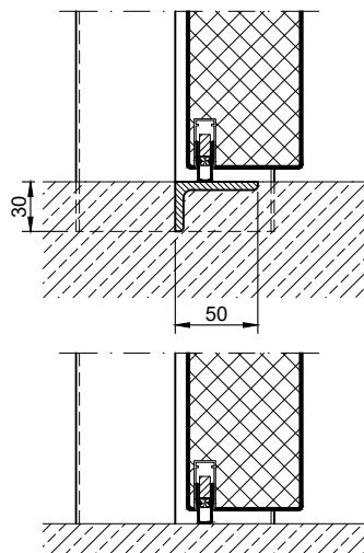
drop seal
